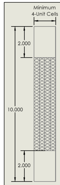
QISO 0-degree Tension Coupon
